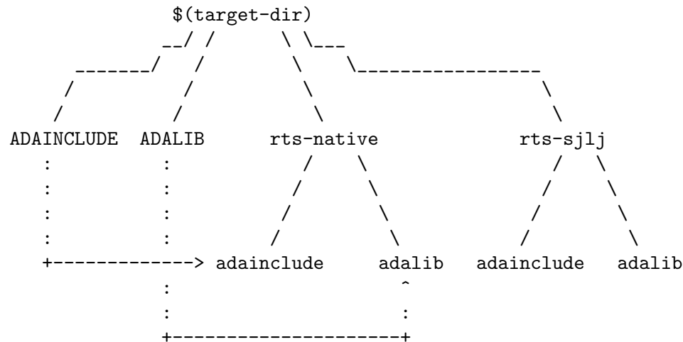
Run-Time Library Directory Structure
